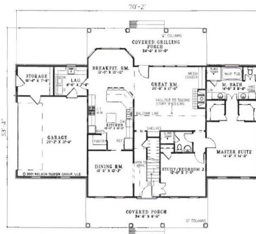
First Floor 1,813 sq. ft.
